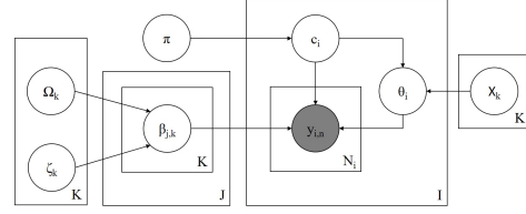
Figure 6: Plate diagram for logistic random effects model.
